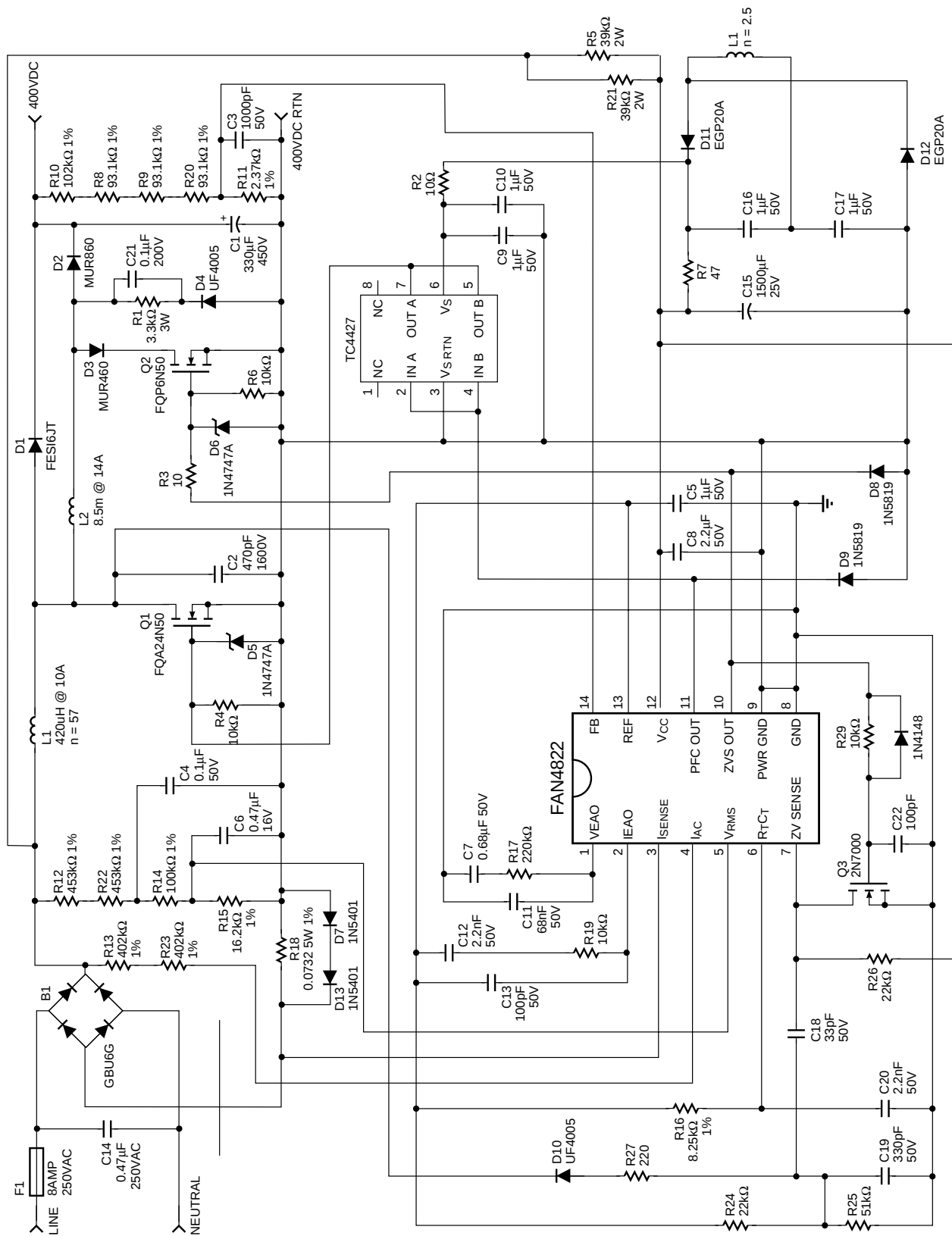
Figure 3. FAN4822 Schematic.
